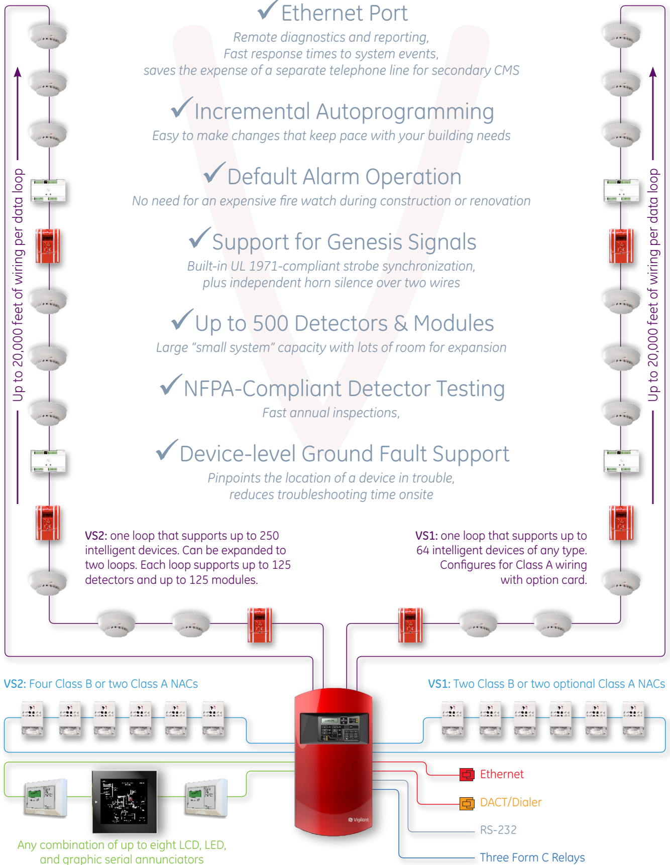
Diagram represents a VS2 system wired for Class A operation with a full complement of option cards.
